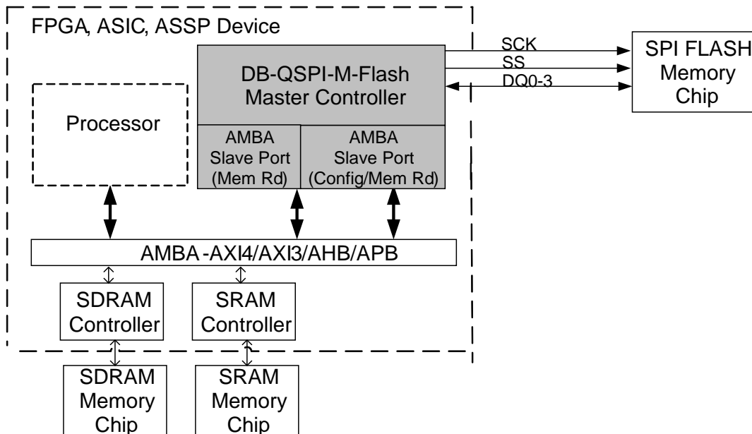
Figure 1: DB-QSPI-FLASH-MEM-AXI Controller – System Diagram
