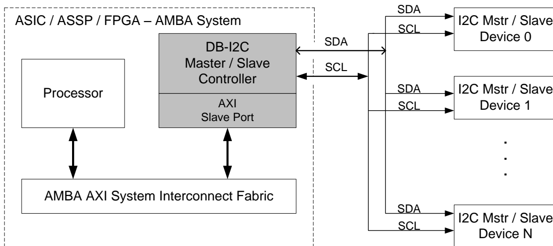
Figure 1: DB-I2C-MS-AXI Controller – System Diagram
