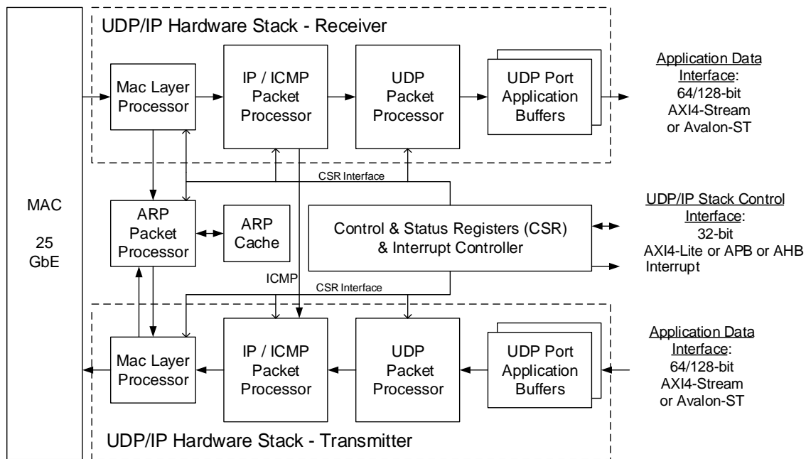
Figure 1: DB-UDP-IP-25GbE-AMBA - Verilog SoC IP Core
